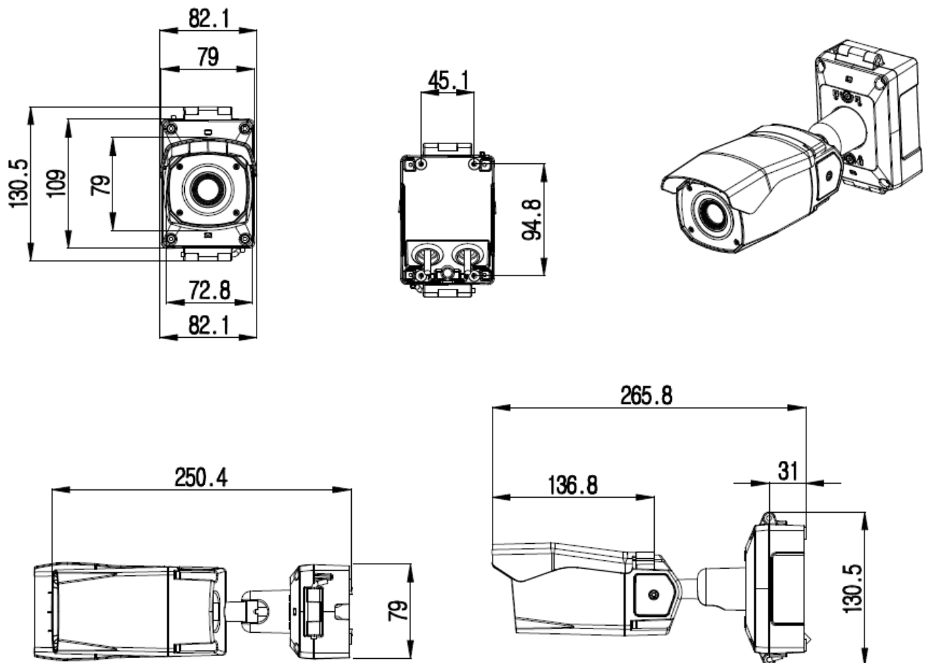
Bullet Type Camera Dimension (unit : mm)
