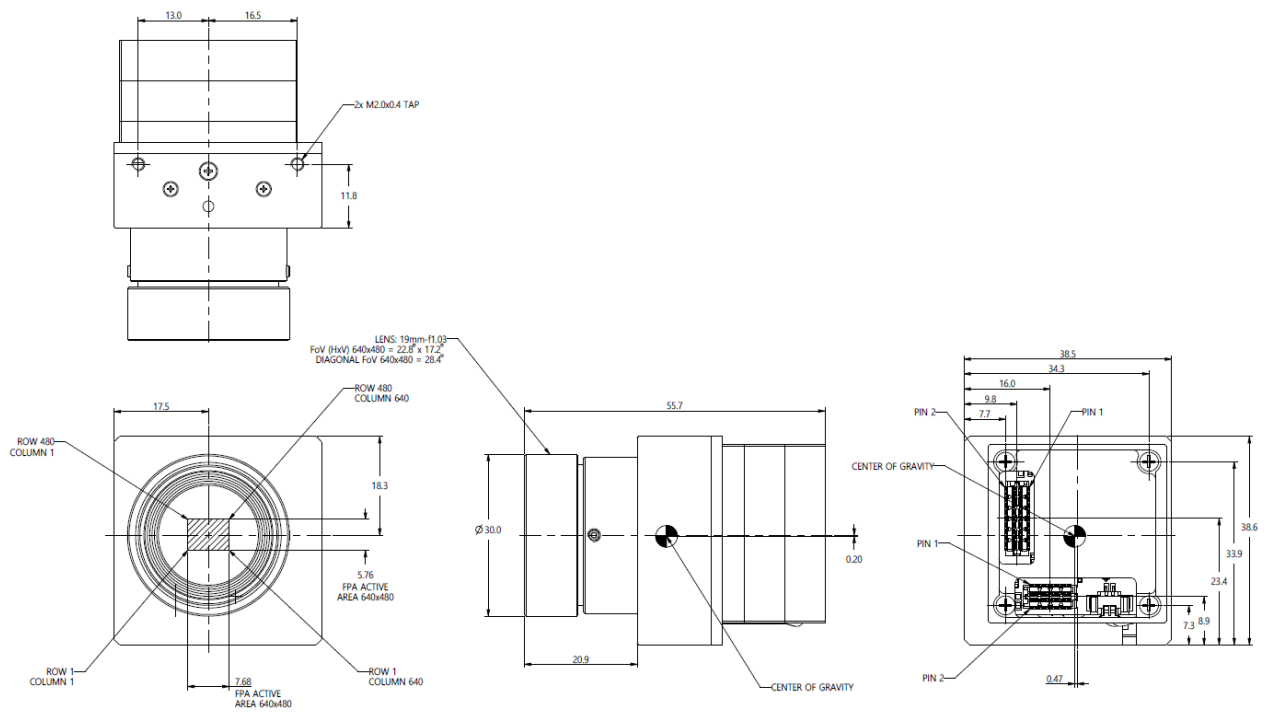
QuantumRed VR(19mm lens) Base Module Dimension (unit : mm)
